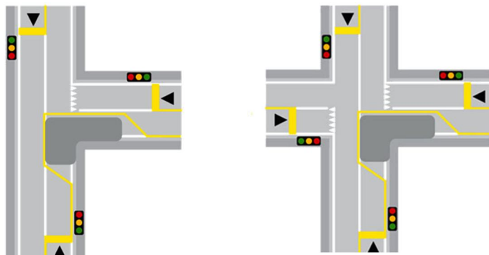
EXAMPLE USE OF 3 OR 4 TRAFFIC LIGHT WITH "MPB" CONTROLLER CODE SPMB0709
